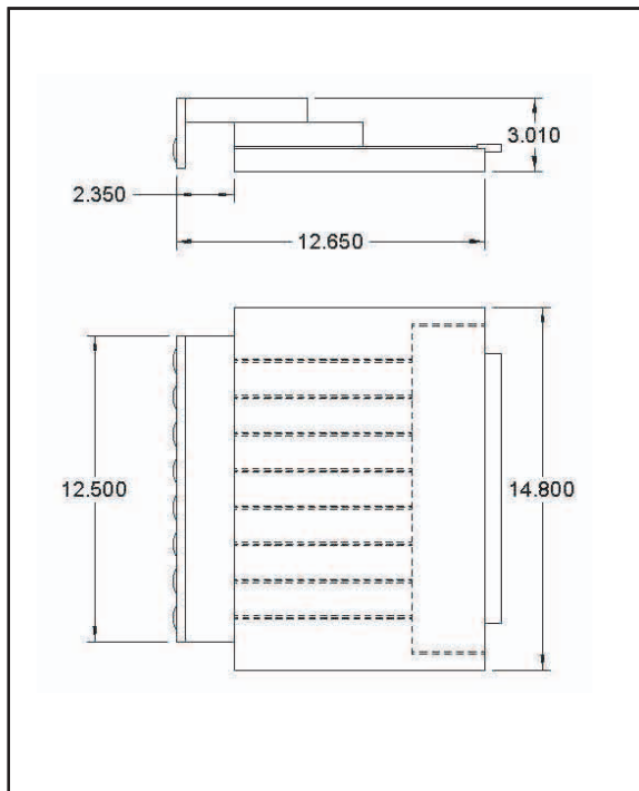
1x8 Lensed Fiber Array (without Housing)
