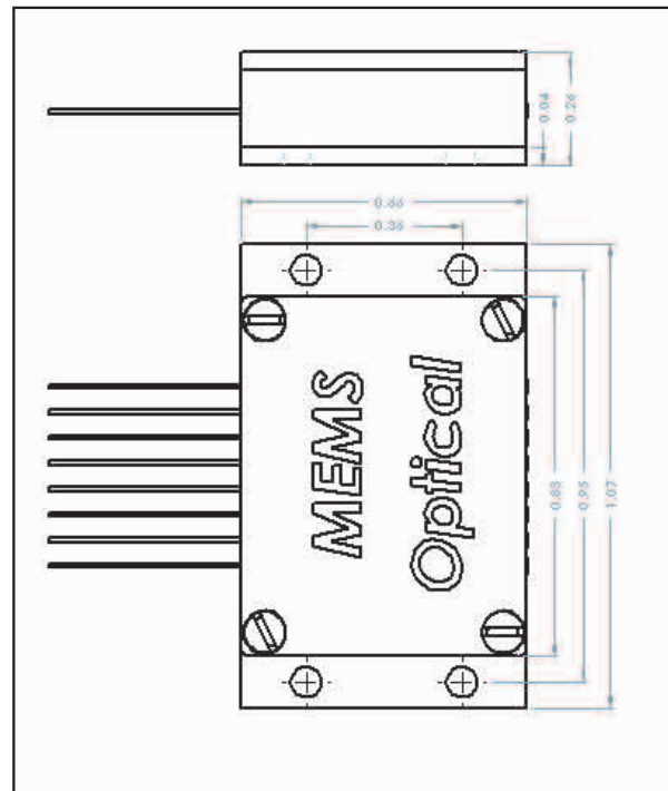
1x8 Lensed Fiber Array (with Housing)
